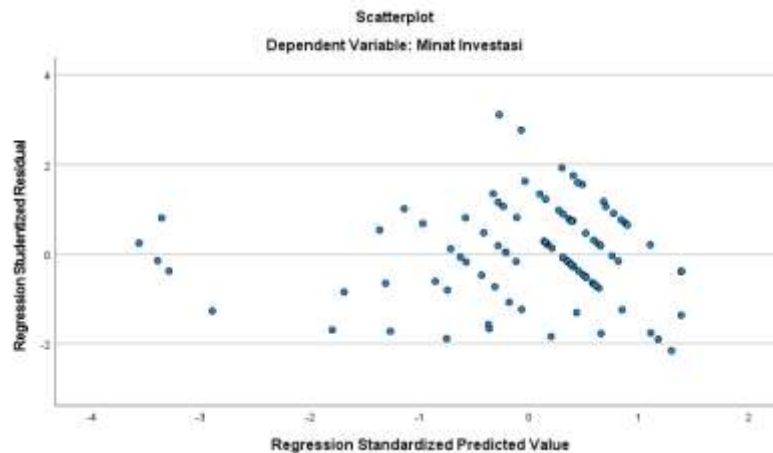
Gambar .2 Scatterplot
